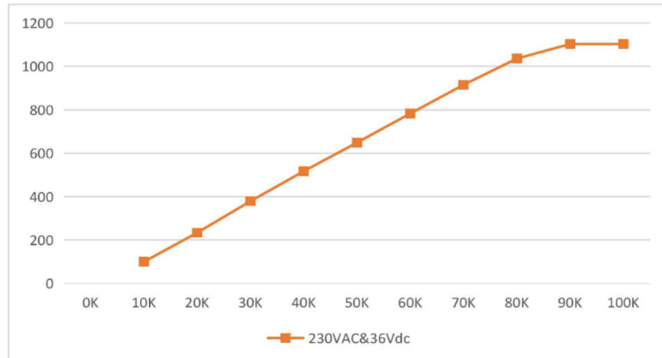
Dimming Curve
