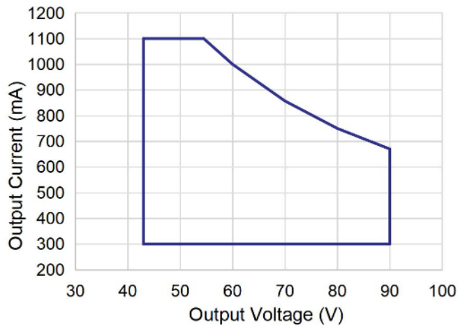
Operating Window
