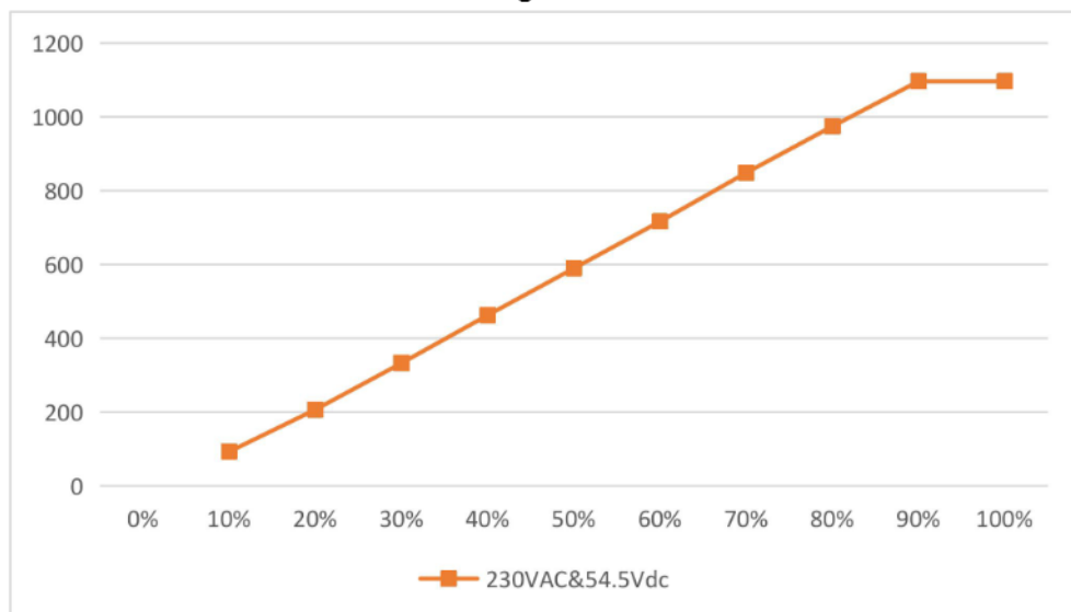
Dimming Curve
