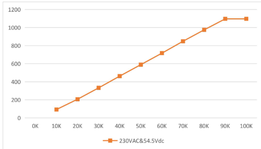
Dimming Curve
