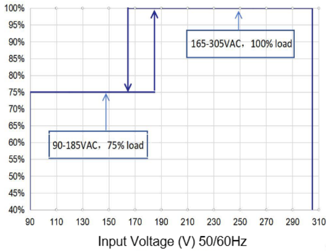
Load Derating Curve
