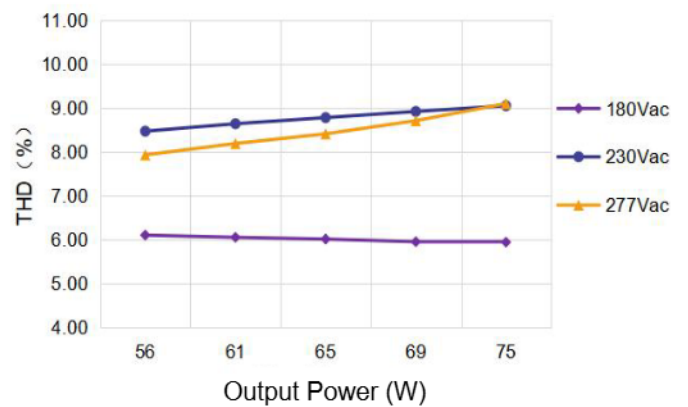
Typical THD vs Load
