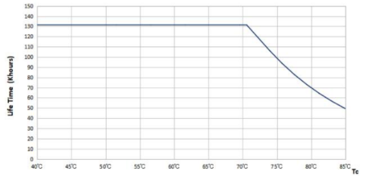
Lifespan
