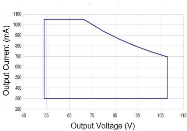
Operating Window
