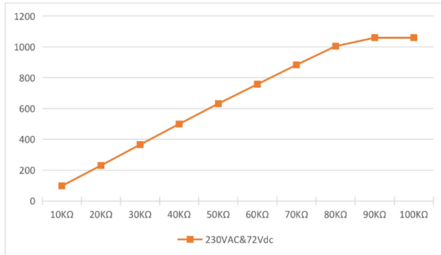
Dimming Curve
