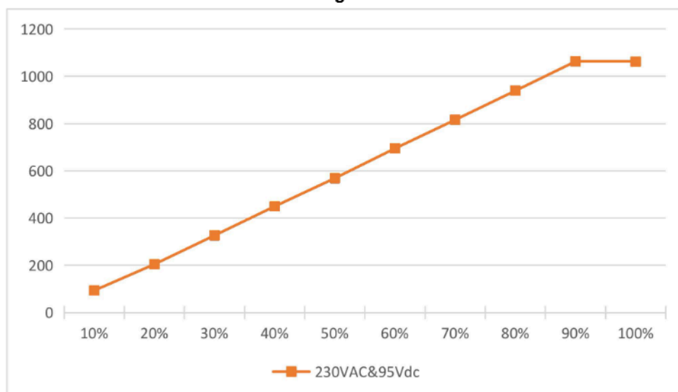
Dimming Curve
