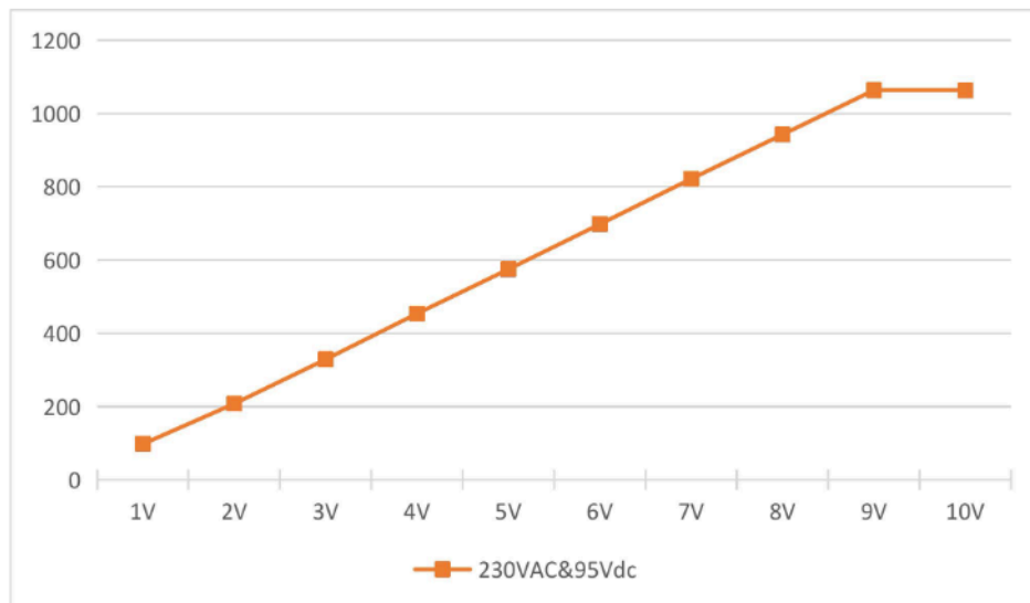
Dimming Curve
