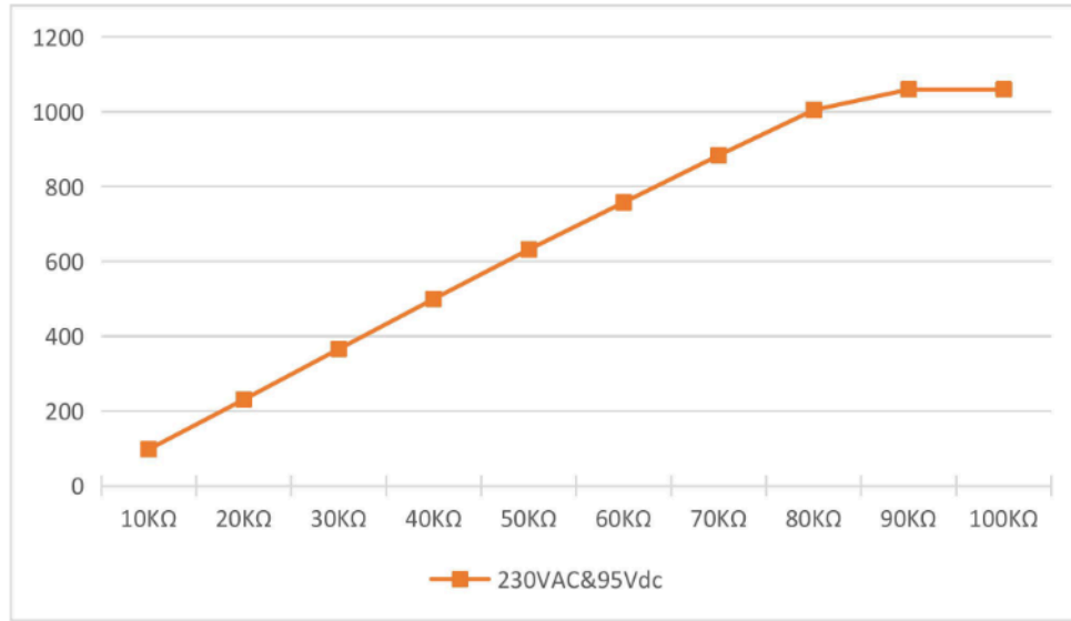
Dimming Curve
