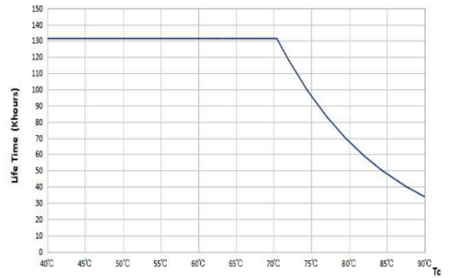
Lifespan
