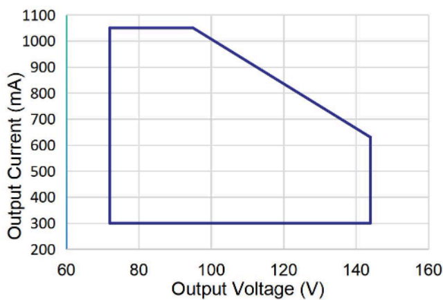
Operating Window
