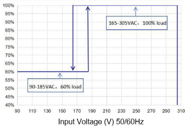
Load Derating Curve
