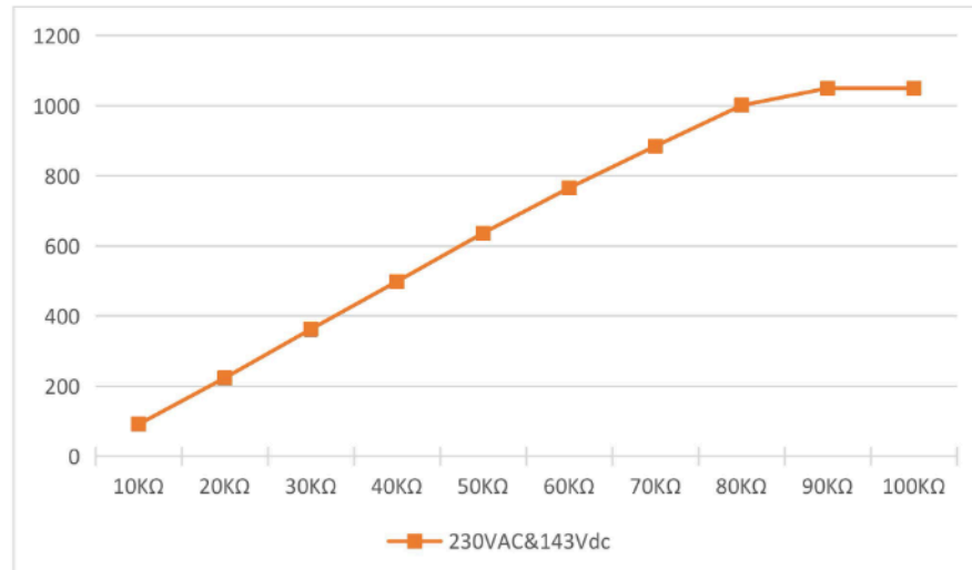
Dimming Curve
