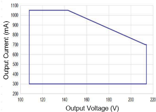
Operating Window
