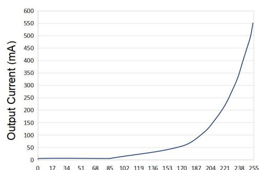
Logarithmic dimming
