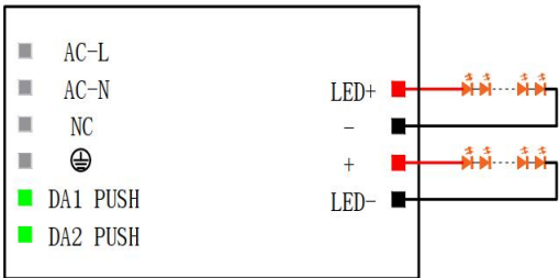
Wiring diagram of double light fixtures
