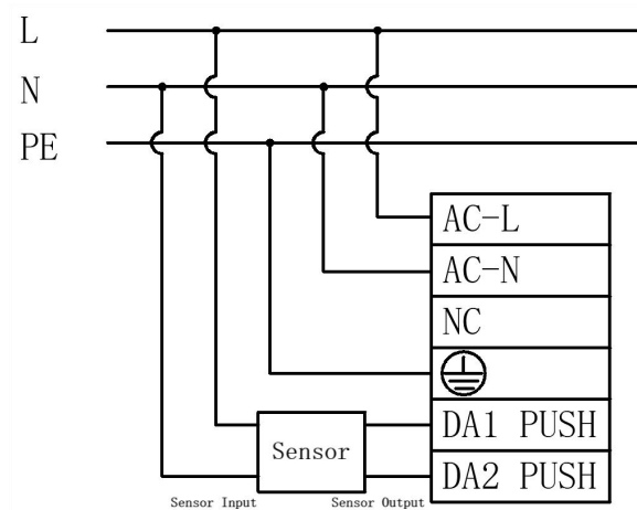
Wiring diagram of corridor dimming
