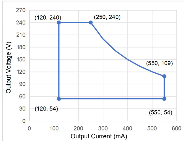
Operating Window
