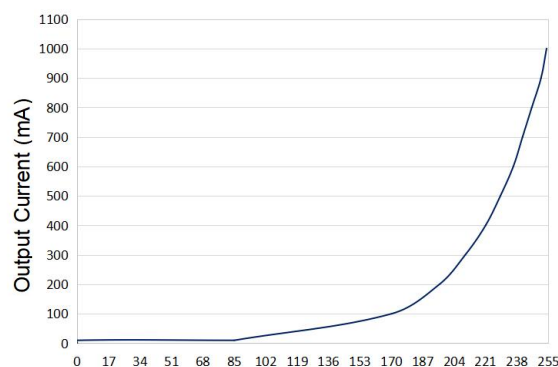
Logarithmic dimming
